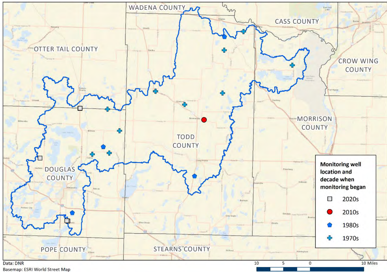
Figure 28: Long Prairie River Watershed – Location of active groundwater level monitoring wells in the Long Prairie River Watershed planning area by decade monitoring started. Twenty wells are measured for groundwater levels in the watershed. Ten of the groundwater level monitoring wells in the watershed has been monitored since the 1970s, four since the 1980s, and the one since the 2010s. Five monitoring wells were installed in 2020.
