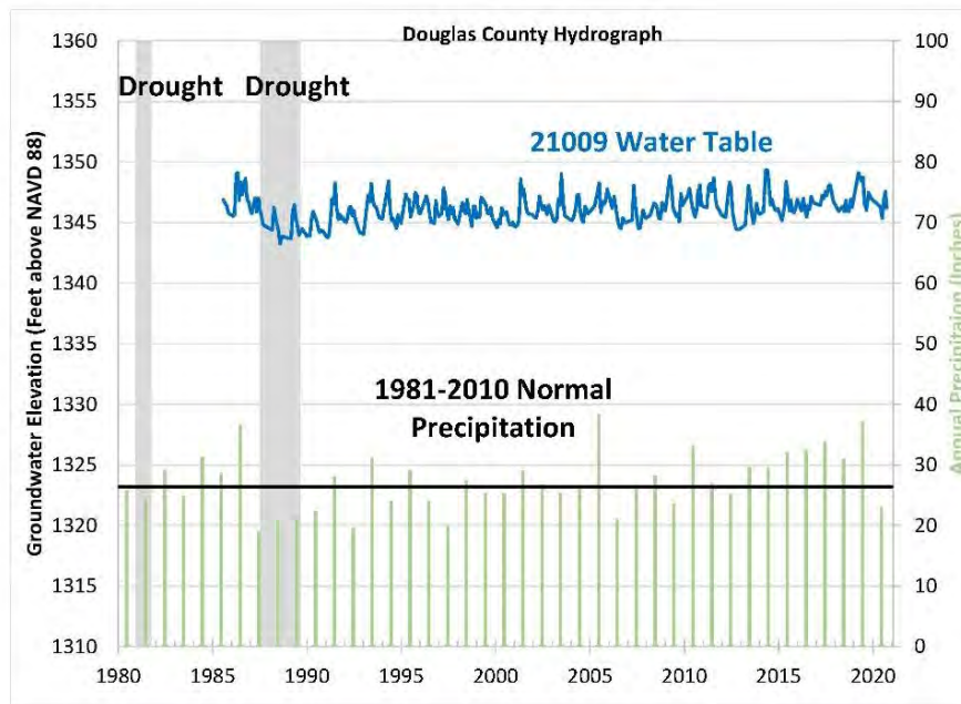
Figure 32: Hydrograph of well 21009 compared with precipitation. The water level in this well has a slight upward trend over the 1990 to 2020 period. The water level declined during the 1988 drought.
