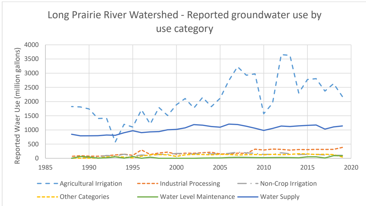
Figure 25: Reported groundwater use from DNR permit holders by use category. Most permitted groundwater withdrawals are used for agricultural irrigation and water supply. Pumping for agricultural irrigation increased from about 1500 million gallons in 1990 to about 3500 million gallons in 2012 and 2013 and then declined slightly. Pumping for water supply was relatively flat at just over 1000 gallons per year.
