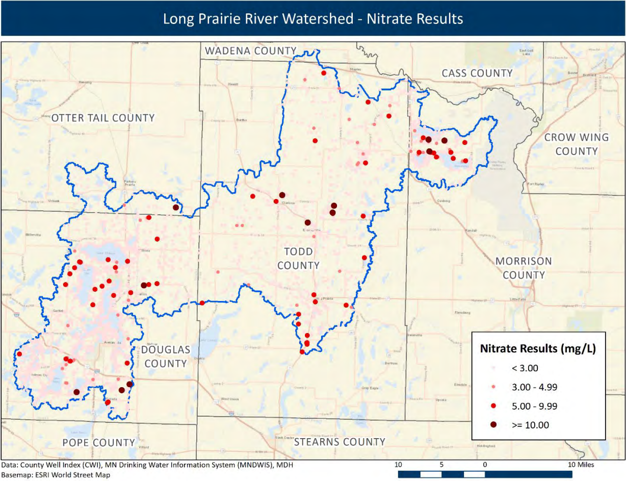
Figure 14: Long Prairie River Watershed - Nitrate results from drinking water wells.
