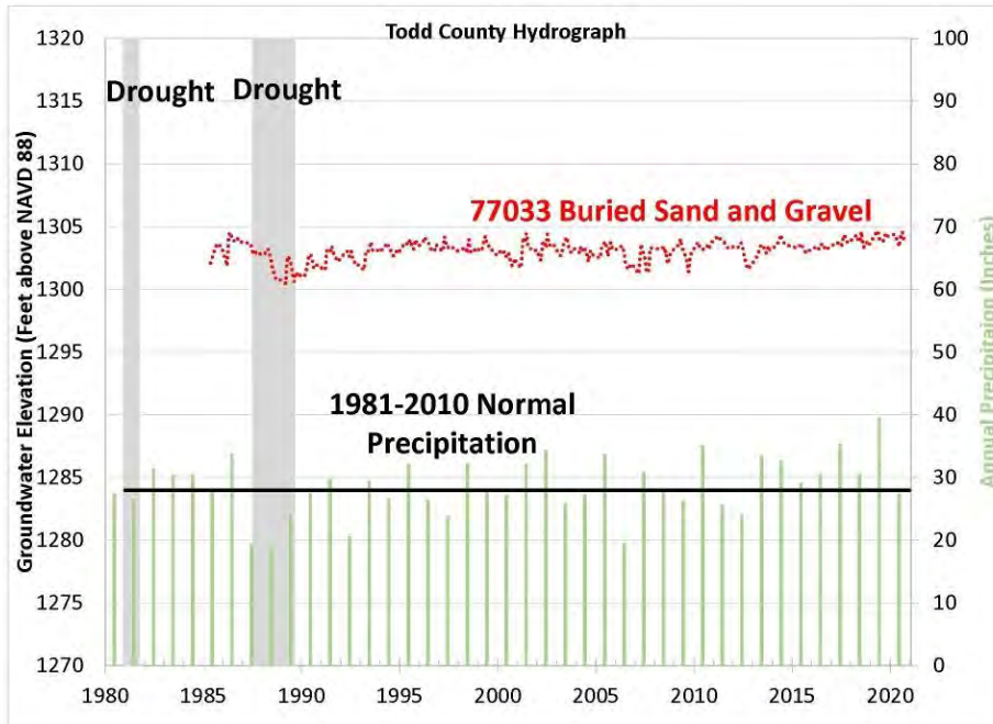
Figure 37: Hydrograph of well 77033 compared with precipitation. The water level in this well has an upward trend over the 1990 to 2020 period.
