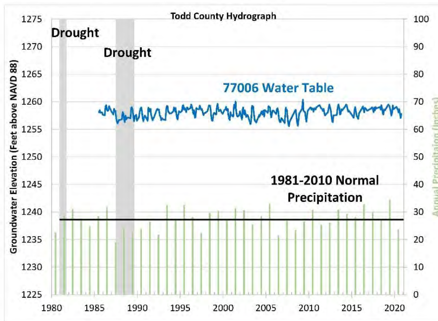
Figure 33: Hydrograph of well 77006 compared with precipitation. The water level in this well has no trend over the 1990 to 2020 period.
