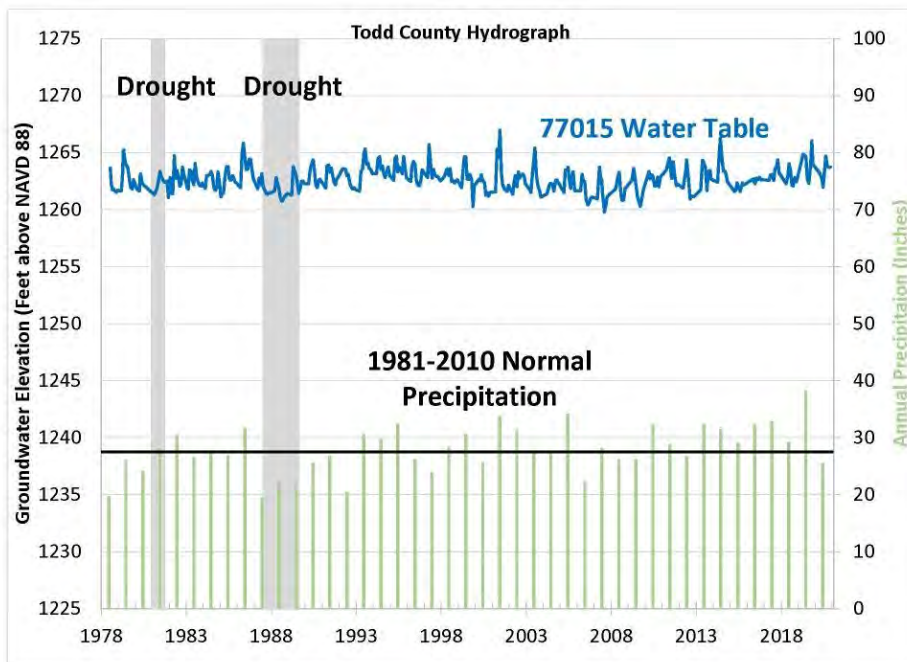
Figure 35: Hydrograph of well 77015 compared with precipitation. The water level in this well has no trend over the 1990 to 2020 period.
