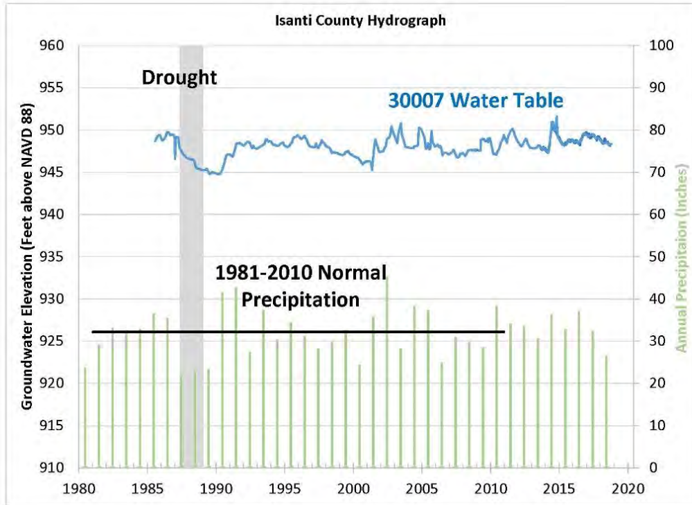
Figure 35: Hydrograph of Obwell 30007 compared with precipitation. The water level has an upward trend for the period 1998-2018 and it varies with precipitation.
