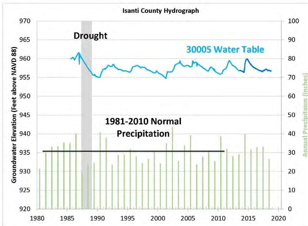
Figure 34: Hydrograph of Obwell 30005 compared with precipitation. The water level varies with precipitation and has no long-term statistical trend.
