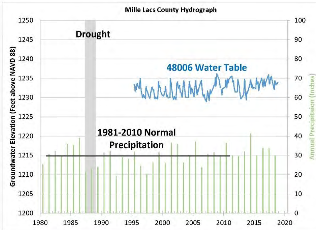
Figure 31: Hydrograph of well 48006 compared to precipitation. The water level has an upward trend over the period 1998-2018.
