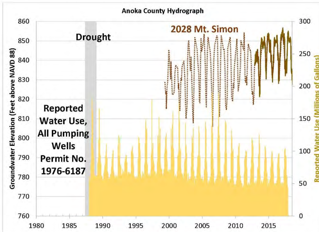
Figure 39: Hydrograph of Obwell 02028 vs. permitted pumping. The water level in this well appears to be rising over the long term, but the period of record is too short to calculate a statistical trend. The annual variations in water level of more than 40 feet is directly related to nearby pumping of municipal wells.
