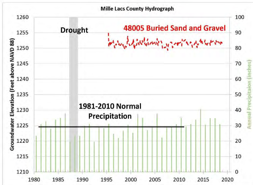
Figure 30: Hydrograph for well 48005 compared to precipitation. The water level has no trend over the period 1998-2018.
