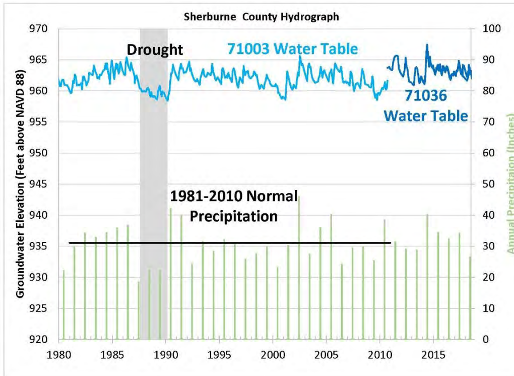
Figure 33: Hydrograph of Obwells 71036 and 71003 compared with precipitation. Well 71036 replaced well 71003, which was sealed. There is no statistical trend in water levels over the period 1998-2018.
