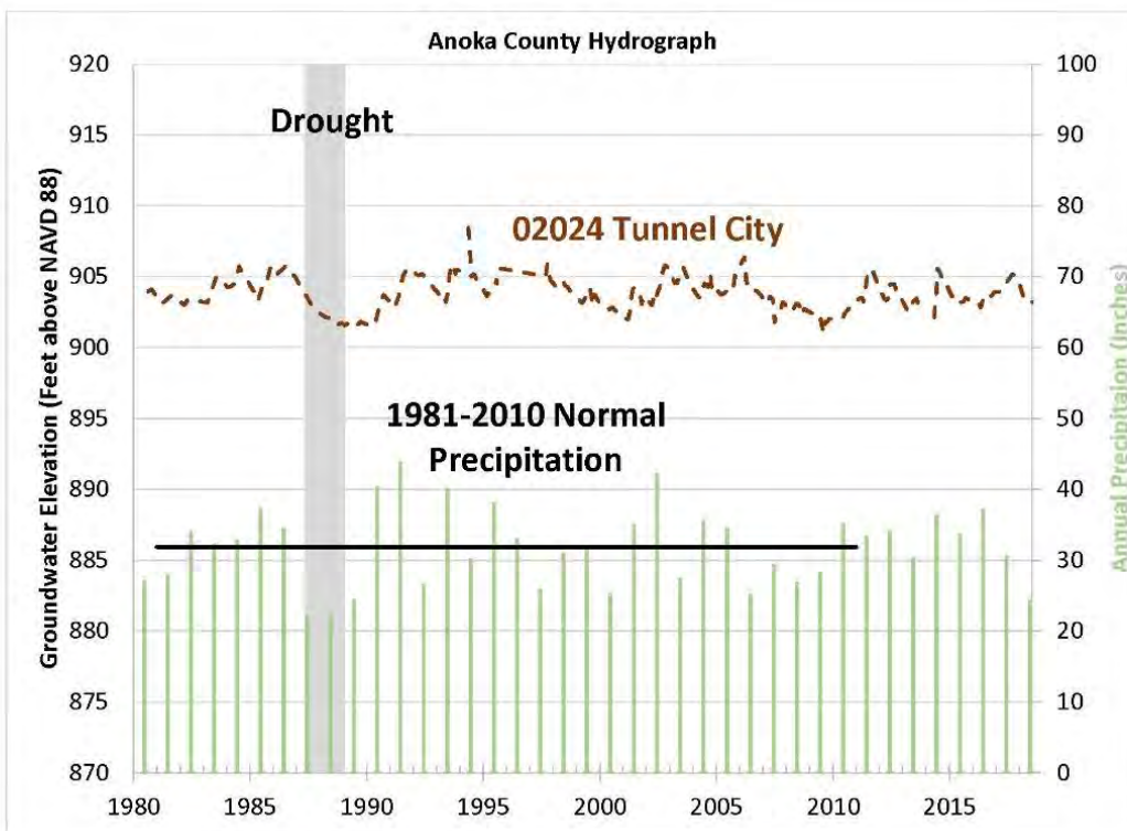
Figure 38: Hydrograph of Obwell 02024 compared with precipitation. The water level varies with precipitation and has no long-term statistical trend.
